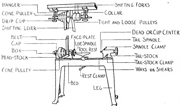
FIG. 200. LATHE—COUNTERSHAFT OVERHEAD.
